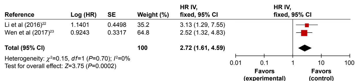
Figure 3 Forest plots of studies evaluating HRs of high UCA1 expression as compared to low expression.
