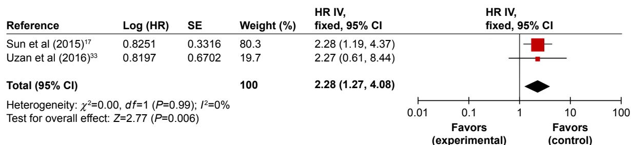
Figure 5 Forest plots of studies evaluating HRs of high HULC expression as compared to low expression.
