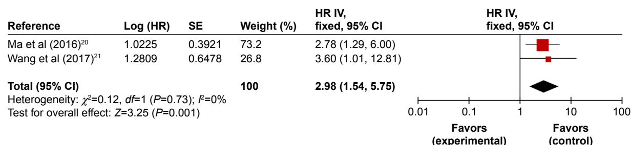
Figure 2 Forest plots of studies evaluating HRs of high TUG1 expression as compared to low expression.
