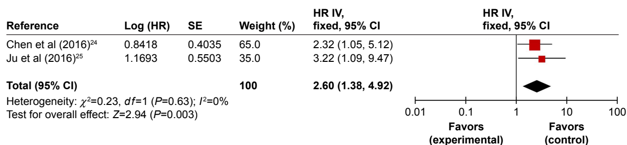
Figure 4 Forest plots of studies evaluating HRs of high BCAR4 expression as compared to low expression.
