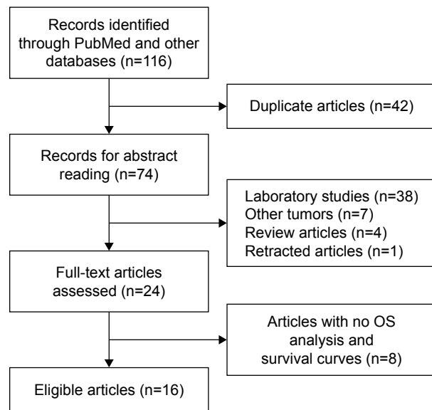
Figure 1 The flowchart of the selection process.
