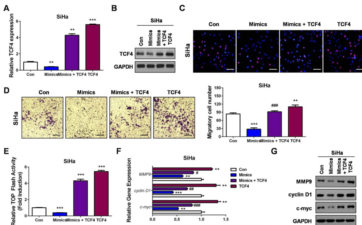
Figure 5 Restoration of TCF4 attenuates the suppressive roles of miR-139-5p in CC progression and recovers the Wnt/β-catenin signaling activity. (A) SiHa cells were transfected with miR-139-5p mimics (Mimics), miR-139-5p mimics plus TCF4 expression plasmids (Mimics+TCF4), TCF4 expression plasmids (TCF4) or controls (Con). 24 hrs later, qRT-PCR was performed to detect the mRNA expression of TCF4. (B) SiHa cells were transfected with miR-139-5p mimics (Mimics), miR-139-5p mimics plus TCF4 expression plasmids (Mimics+TCF4), TCF4 expression plasmids (TCF4) or controls (Con). 24 hrs later, Western blot analysis was performed to detect the protein expression of TCF4. (C) SiHa cells were transfected with miR-139-5p mimics (Mimics), miR-139-5p mimics plus TCF4 expression plasmids (Mimics+TCF4), TCF4 expression plasmids (TCF4) or controls (Con). 24 hrs later, EdU assay was performed to detect the cell proliferation ability. (D) SiHa cells were transfected with miR-139-5p mimics (Mimics), miR-139-5p mimics plus TCF4 expression plasmids (Mimics+TCF4), TCF4 expression plasmids (TCF4) or controls (Con). 24 hrs later, transwell assay was performed to detect the cell migration ability. (E) SiHa cells were co-transfected with TOP Flash firefly luciferase plasmid, renilla luciferase plasmid, miR-139-5p mimics (Mimics) or miR-139-5p mimics plus TCF4 expression plasmids (Mimics+TCF4), TCF4 expression plasmids (TCF4) or controls (Con). 48 hrs later, luciferase activity was determined, and relative Wnt/β-catenin activity was calculated. (F) SiHa cells were transfected with miR-139-5p mimics (Mimics), miR-139-5p mimics plus TCF4 expression plasmids (Mimics+TCF4), TCF4 expression plasmids (TCF4) or controls (Con). 24 hrs later, qRT-PCR was performed to detect the mRNA expressions of Wnt target genes. (G) SiHa cells were transfected with miR-139-5p mimics (Mimics), miR-139-5p mimics plus TCF4 expression plasmids (Mimics+TCF4), TCF4 expression plasmids (TCF4) or controls (Con). 24 hrs later, Western blot analysis was performed to detect the protein expressions of Wnt target genes. Scale bar: 200 μm. ** P < 0.01 , *** P < 0.001 , compared with Con group. # P < 0.05 , ## P < 0.01 , ### P < 0.001 , compared with Mimics group.
